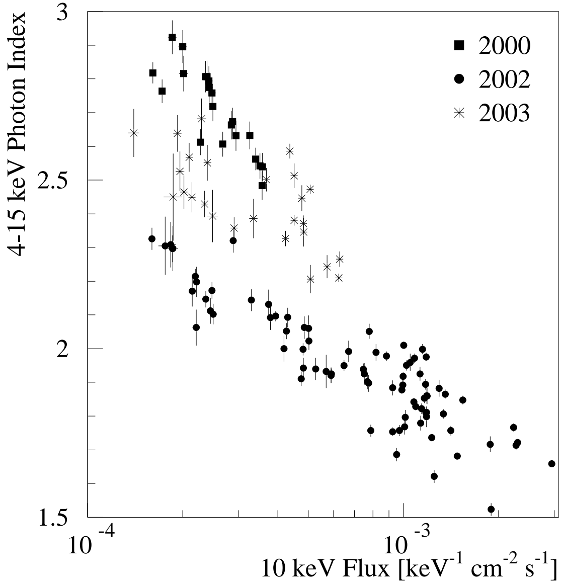
Fig. 3.— Correlation between the X-ray flux and the 4-15 keV photon index for observations in the years 2000, 2002 and 2003.
