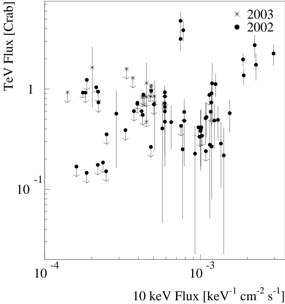
Fig. 2.— Correlation between the X-ray and TeV \gamma -ray fluxes for measurements within two hours of each other.
